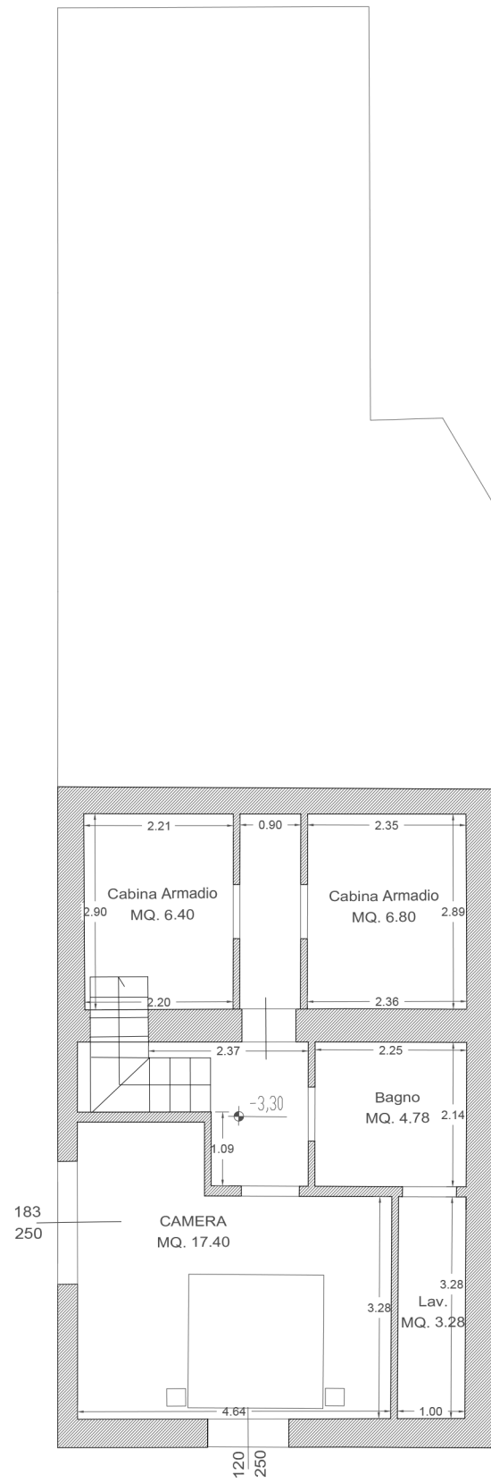
PIANO SEMI-INTERRATO
